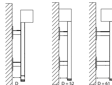
Pose standard
